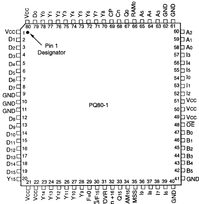
PQFP TOP VIEW
