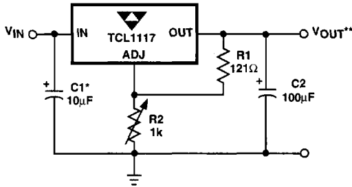
1.2V-10V Adjustable Regulator
