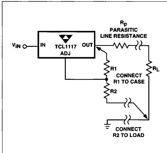
Figure 3. Connections for Best Load Regulation
