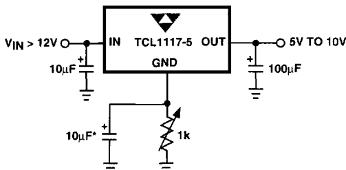
Adjusting Output Voltage of Fixed Regulators
