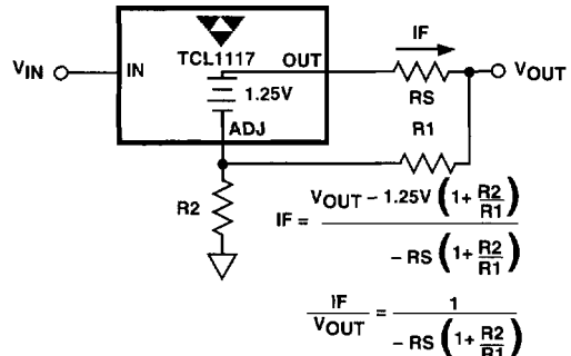
Battery Charger
