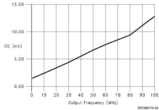
Typical I_{CC} vs Output Switching Frequency, C_L = 0 pF, V_{CC} = V_{IH} = 5.5\text{V} , LE = \text{GND} , 1 Output Switching at 50% Duty Cycle, Data to Output, Transparent Mode with Unused Data Inputs = V_{IH}
