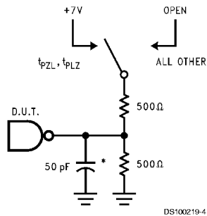
FIGURE 1. Test Load
