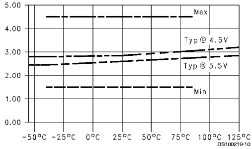
T_{PLH} vs Temperature ( T_A ), C_L = 50 pF, 1 Output Switching, Data to Output
