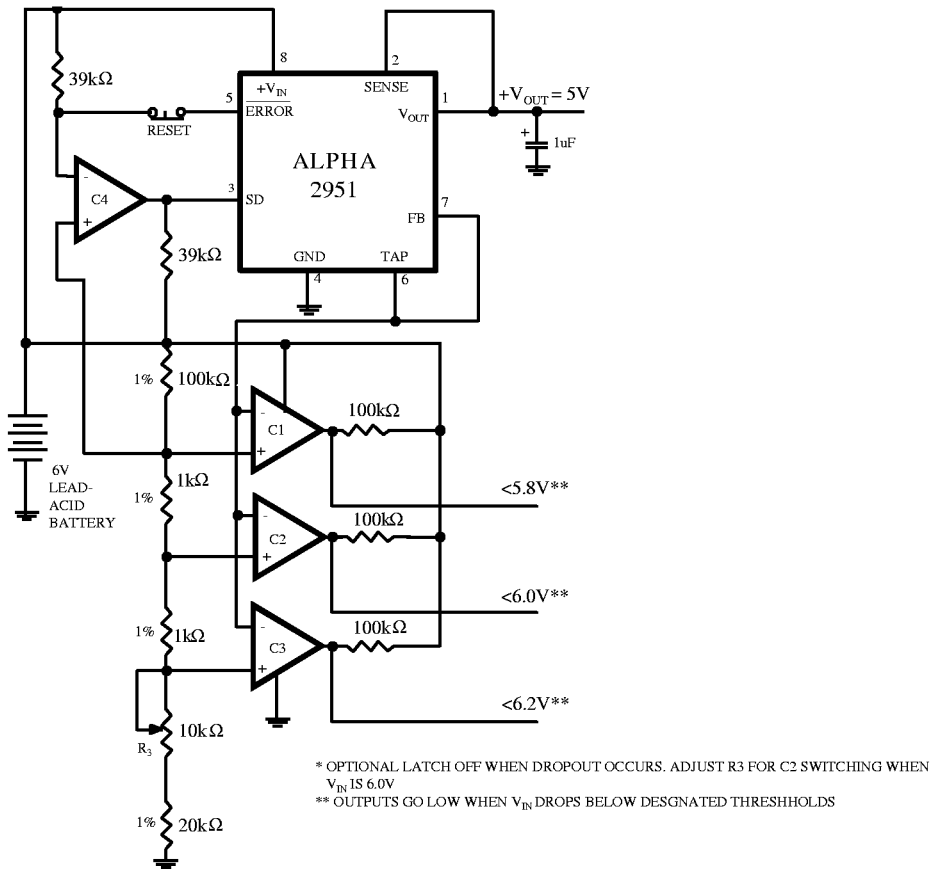
Regulator with State-of-Charge indicator
