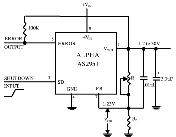
Figure 2. Adjustable Regulator
