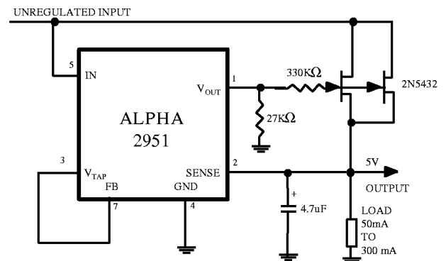
300 mA Regulator with 0.75 Dropout
