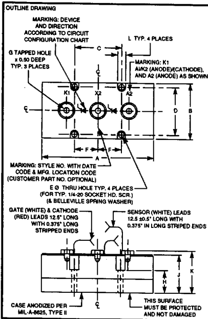
POW-R-BRIK™ Phase Control Modules 345-800 Amperes/400-3000 Volts
