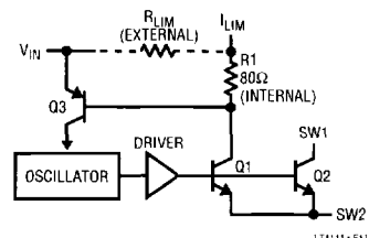
Figure 11. LT1111 Current Limit Circuitry
