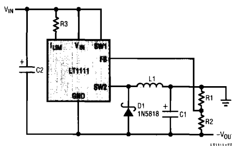
Figure 7. Positive-to-Negative Converter
