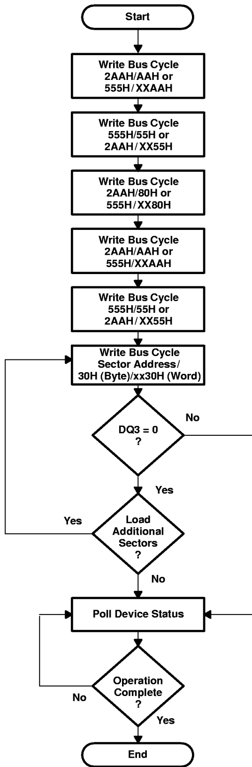
Figure 14. Sector-Erase Algorithm
