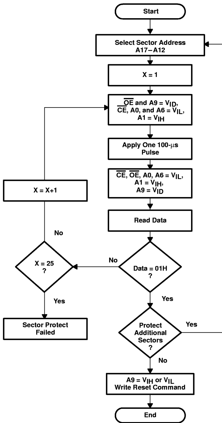
Figure 20. Sector-Protect Algorithm
