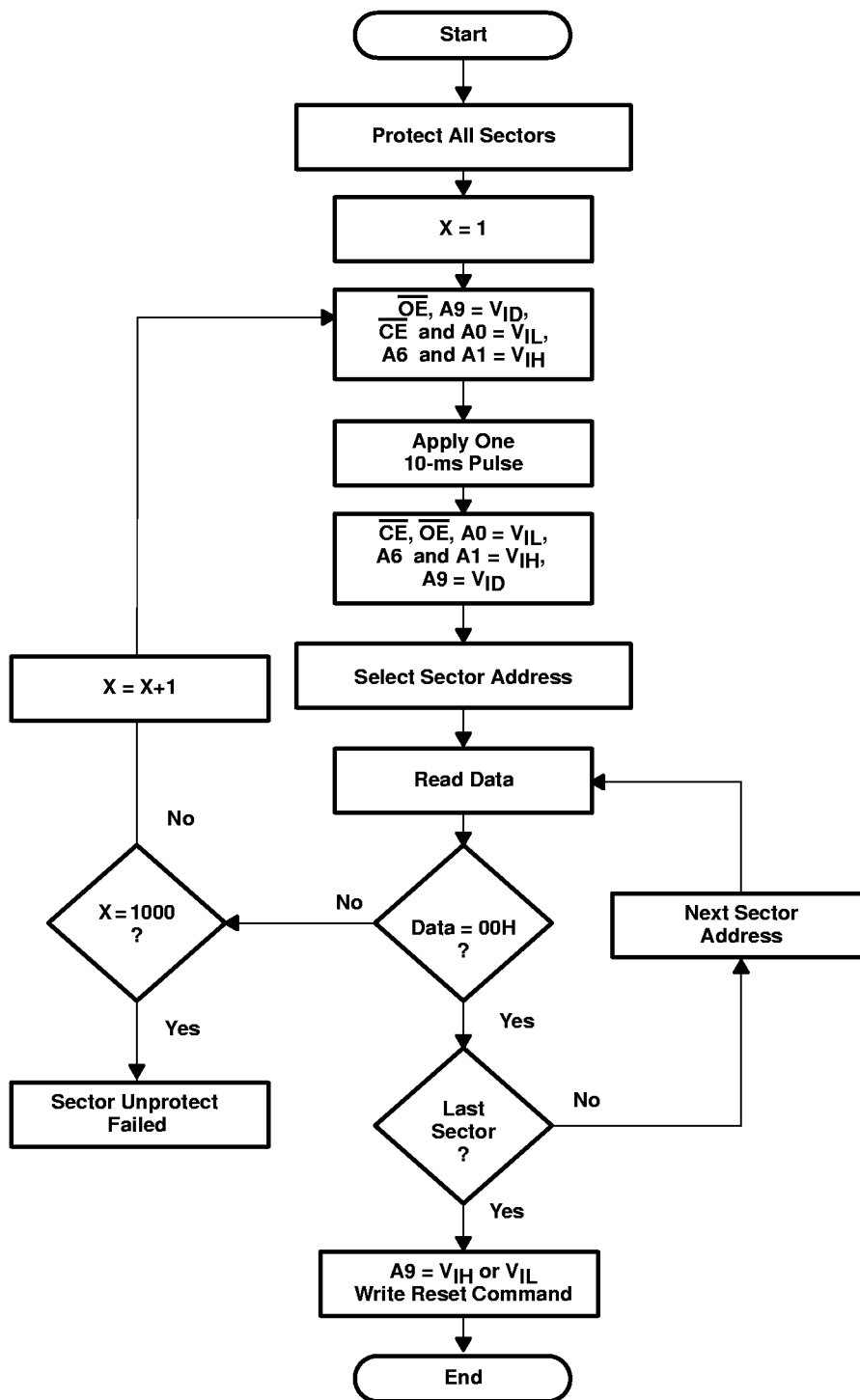
Figure 22. Sector-Unprotect Algorithm
