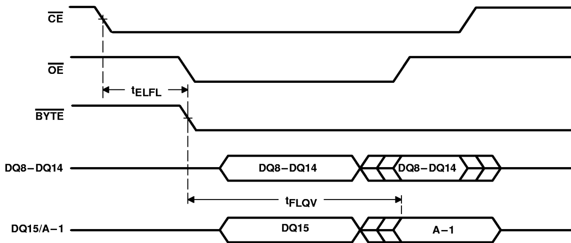
Figure 4. Byte-Mode Configuration
