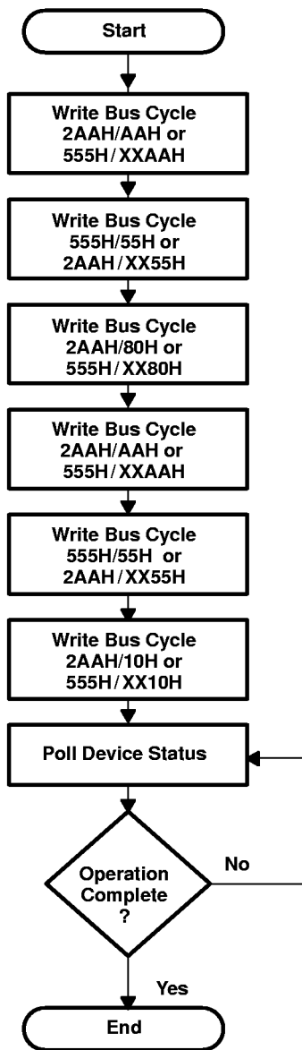
Figure 12. Chip-Erase Algorithm
