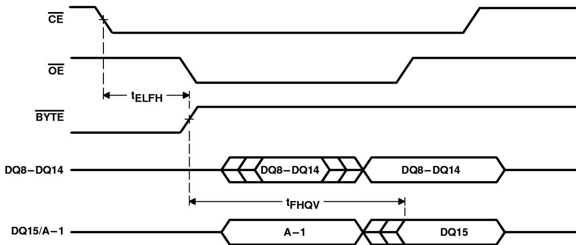
Figure 3. Word-Mode Configuration
