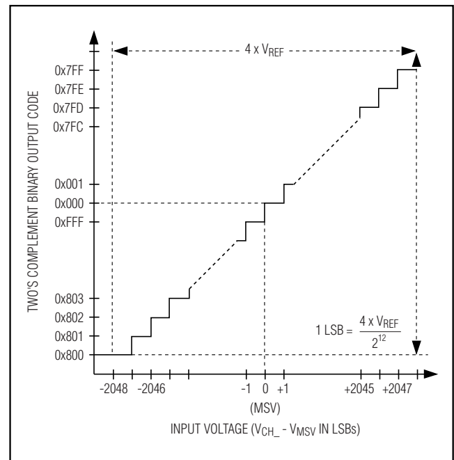
Figure 9. \pm 5V Bipolar Transfer Function
