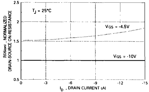
Figure 4. On-Resistance Variation with Drain Current
