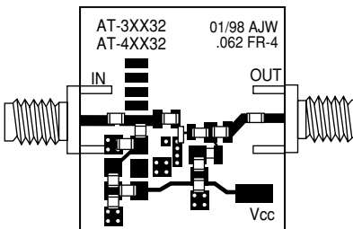
Figure 18. IX Artwork showing Component Placement.
