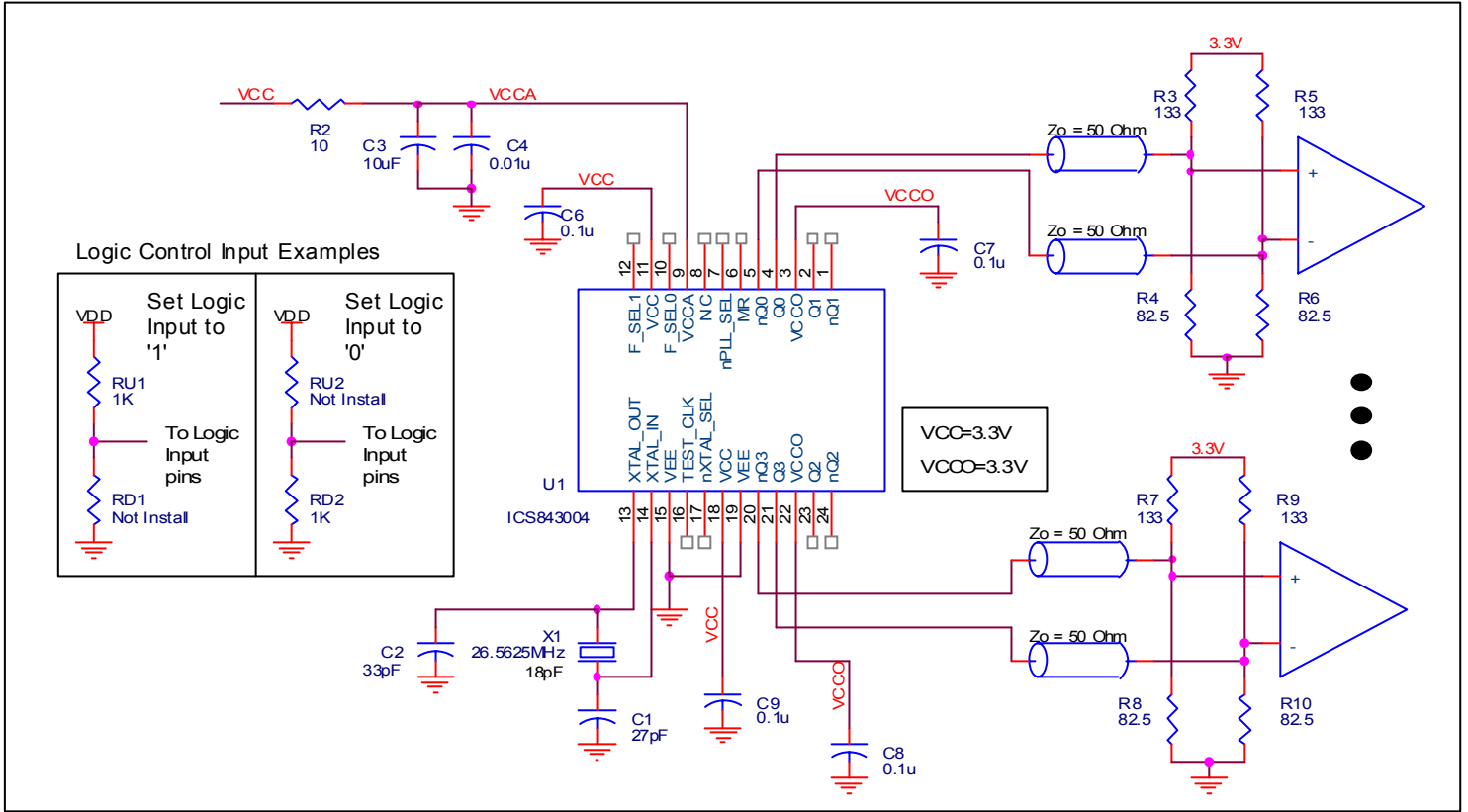
Figure 6. ICS843004I Schematic Example
