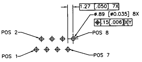
VIEW C SCALE 2/1 TYPICAL FOOTPRINT
