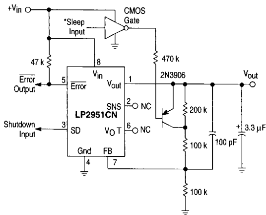
Figure 21. 5.0 V Regulator with 2.5 V Sleep Function
