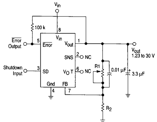
Figure 16. Adjustable Regulator
