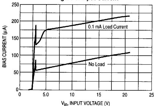
Figure 3. Input Current
