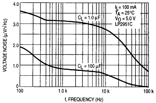
Figure 12. Output Noise
