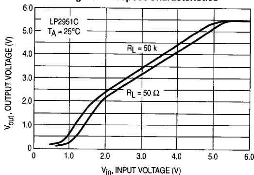
Figure 2. Dropout Characteristics
