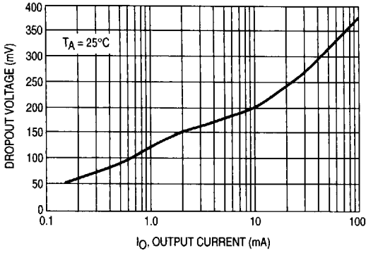
Figure 5. Dropout Voltage versus Output Current
