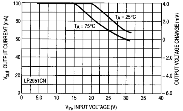
Figure 14. Maximum Rated Output Current
