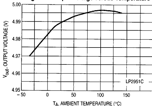
Figure 4. Output Voltage versus Temperature
