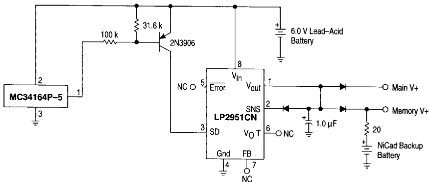
Figure 25. Low Battery Disconnect
