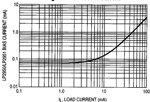
Figure 1. Quiescent Current
