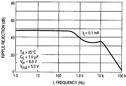
Figure 11. Ripple Rejection
