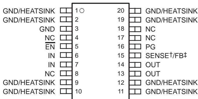
PWP PACKAGE (TOP VIEW)
