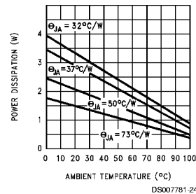
Maximum Power Dissipation (TO-263) (See Note 2)
