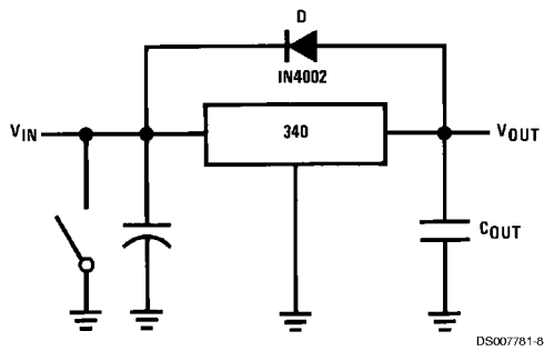
FIGURE 1. Input Short
