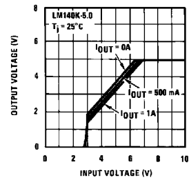
Dropout Characteristics
