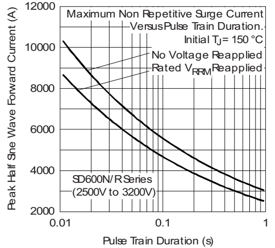
Fig. 12 - Maximum Non-Repetitive Surge Current
