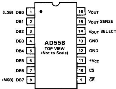
D Package (DIP)
