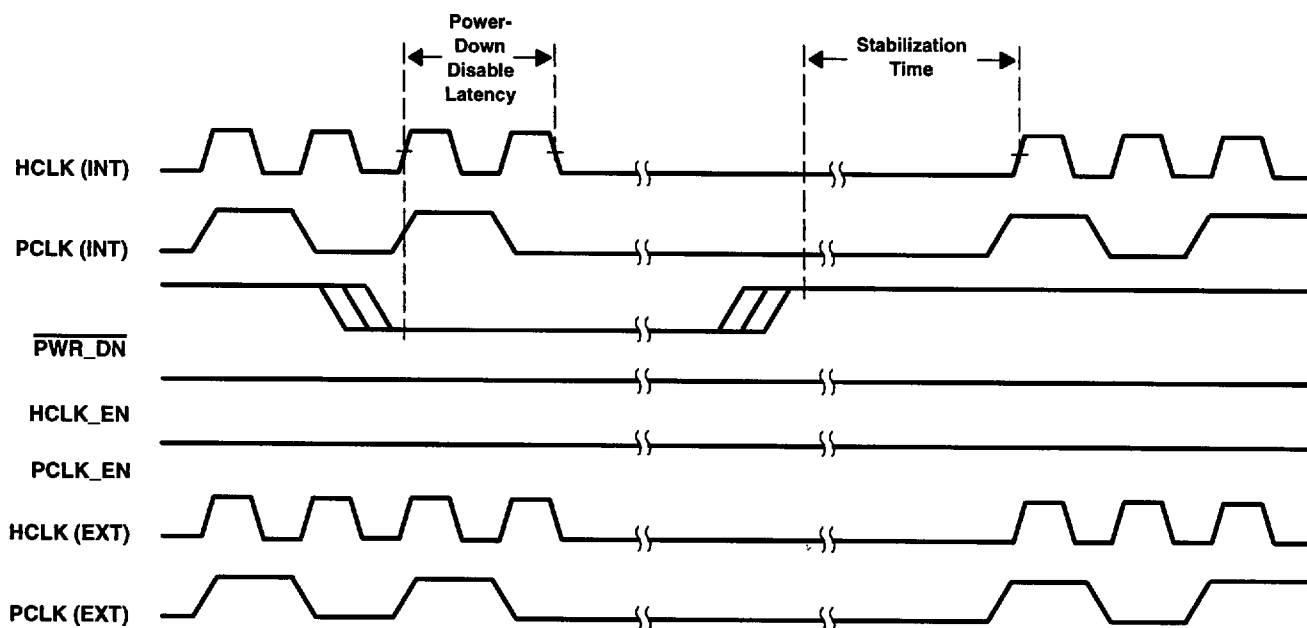
Figure 4. Power-Down Timing
