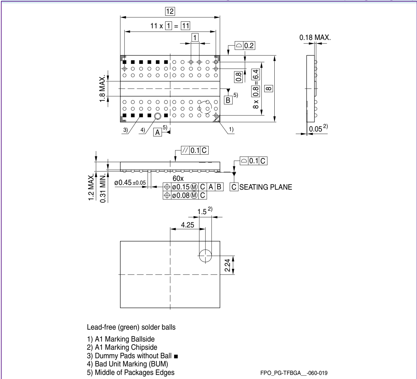
FIGURE 4 Package Outline of P-TFBGA-60-12 (non-green/green)
