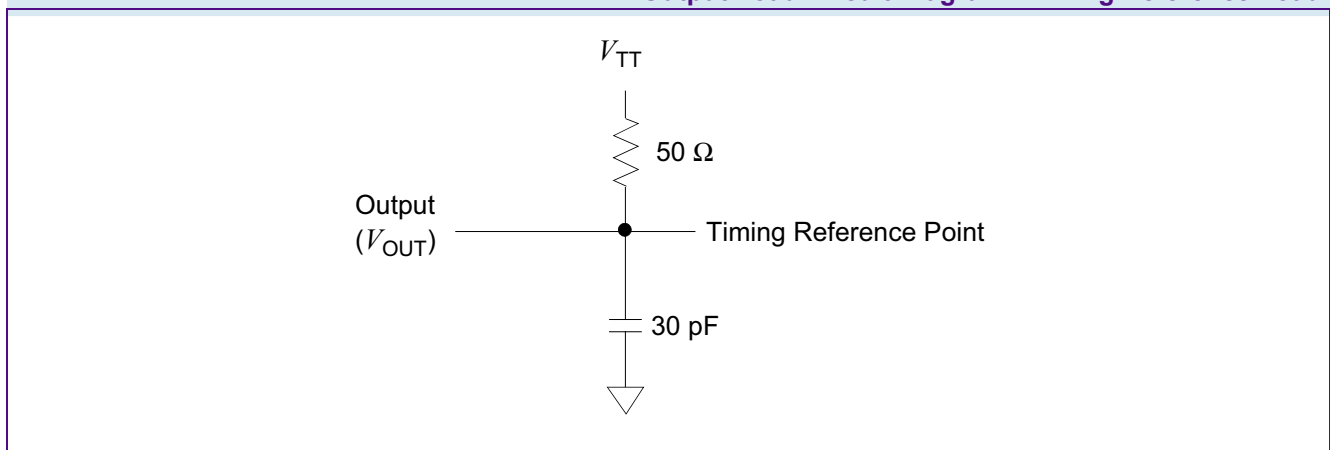
AC Output Load Circuit Diagram / Timing Reference Load
