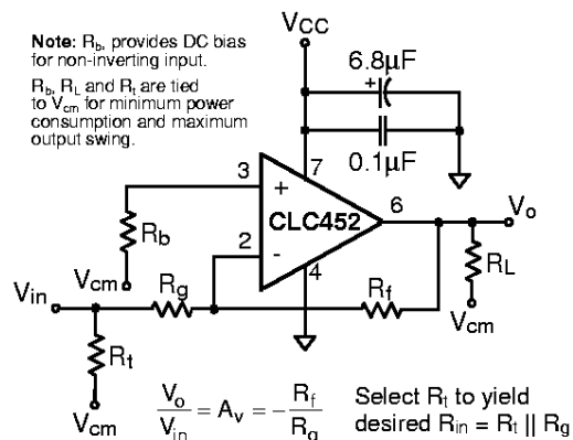
Figure 2: Inverting Configuration
