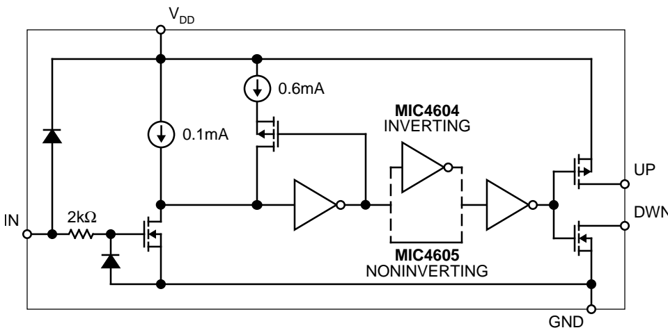
Functional Diagram for One Driver (Two Drivers per Package—Ground Unused Inputs)
