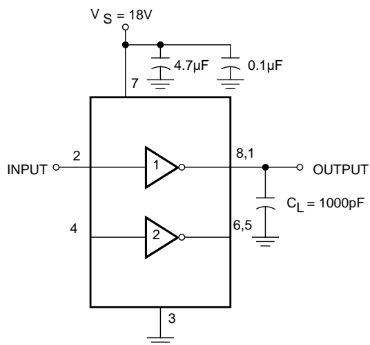
Figure 1. MIC4604/4605 Switching time test circuit.
