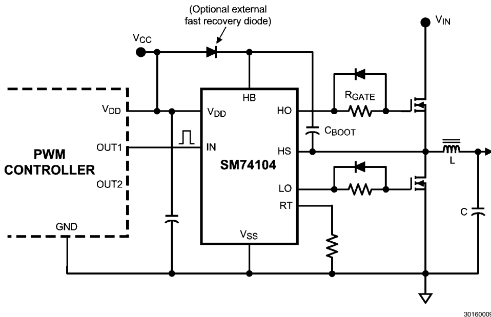
FIGURE 2. SM74104 Driving MOSFETs Connected in Synchronous Buck Configuration
