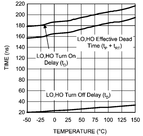
Timing vs Temperature RT = 100K
