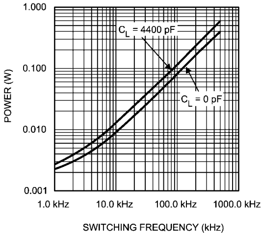
Diode Power Dissipation V_{IN} = 80V
