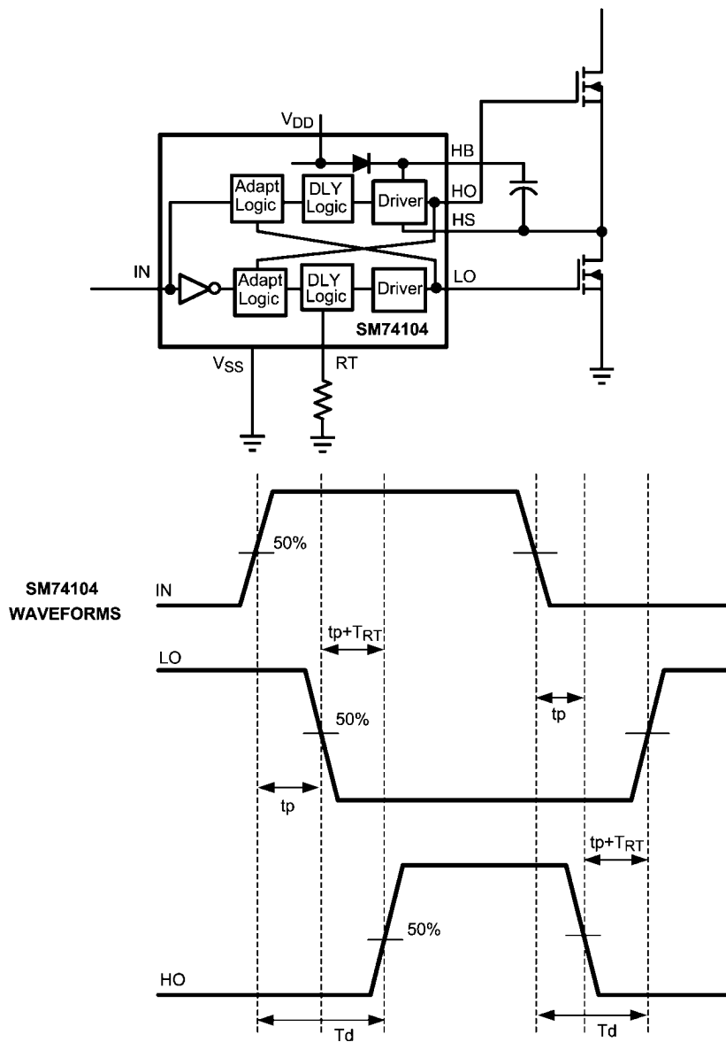
FIGURE 1. Application Timing Waveforms
