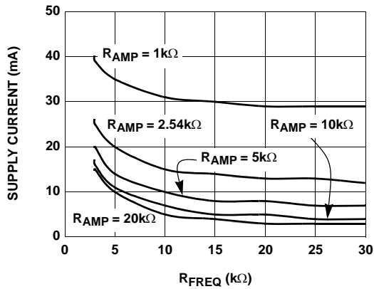
FIGURE 7. SUPPLY CURRENT vs R_{FREQ}
