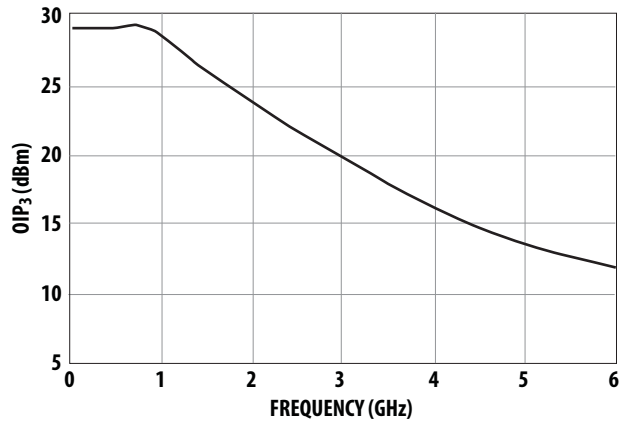
Figure 5. OIP_3 vs. Frequency at I_d = 35 mA.
