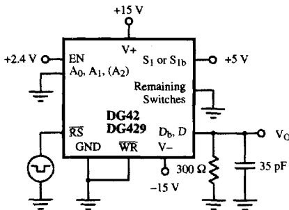
Figure 8. Reset Turn-Off Time ( t_{OFF(RS)} )
