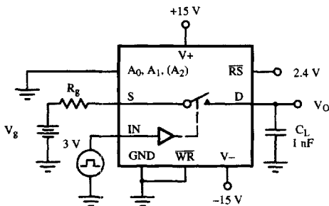
Figure 9. Charge Injection
