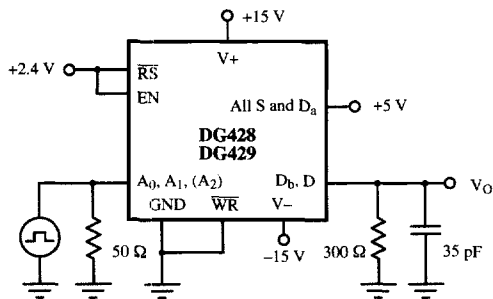
Figure 4. Break-Before-Make
