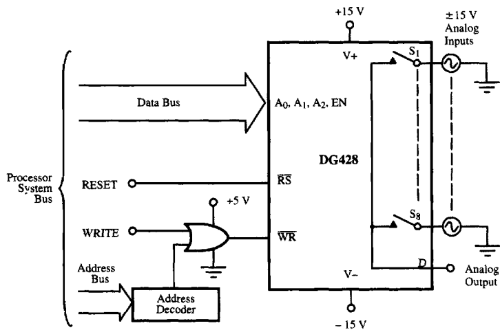
Figure 10. Bus Interface
