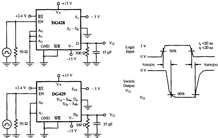
Figure 6. Enable t_{ON}/t_{OFF} Time
