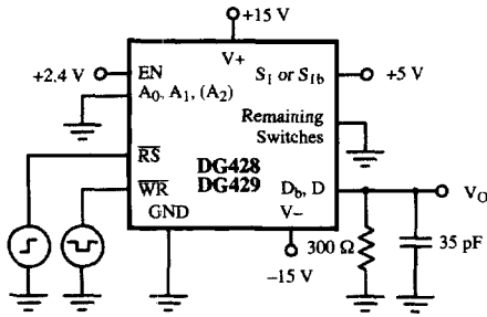
Figure 7. Write Turn-On Time ( t_{ON(WR)} )
