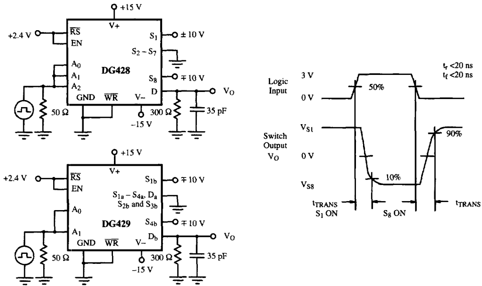
Figure 5. Transition Time
