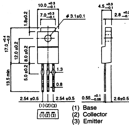
2SD1889 (TO-220FP)
