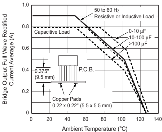
Figure 1. Derating Curves Output Rectified Current for B40C800G...B125C800G
