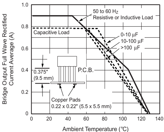
Figure 2. Derating Curves Output Rectified Current for B250C800G...B380C800G
