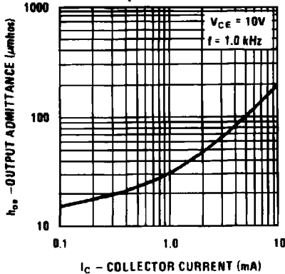
Output Admittance
