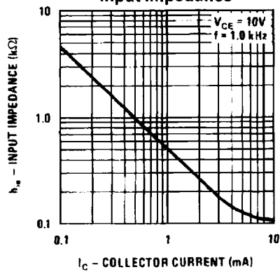
Input Impedance
