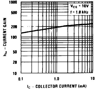
Current Gain
