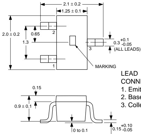
PACKAGE OUTLINE 33
