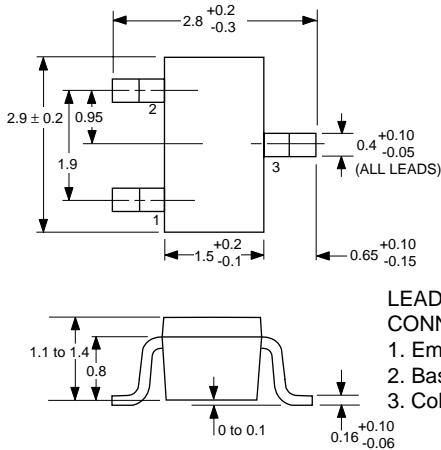
PACKAGE OUTLINE 33
