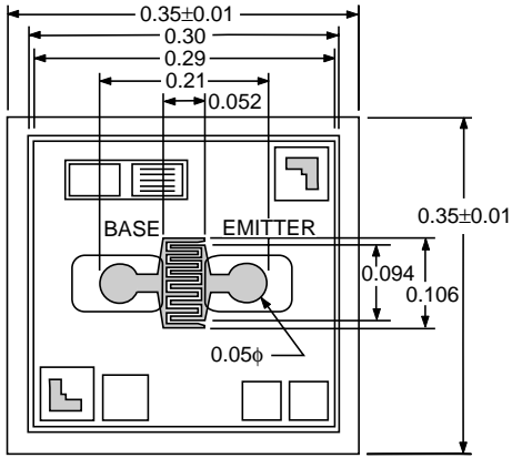
NE02100 (CHIP)
