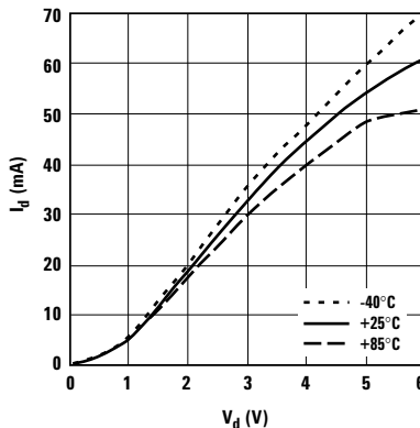
Figure 9. Current vs. Voltage and Temperature.
