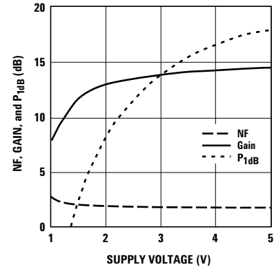
Figure 3. Gain, NF and P1dB vs. supply voltage at 1900 MHz.
