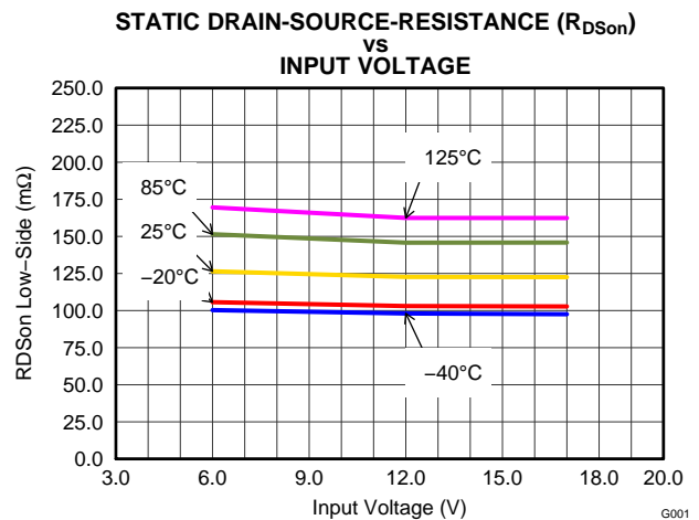
Figure 20. Low-Side Switch
