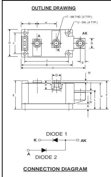
ND412235 Dual Diode Isolated POW-R-BLOK™ Module 200-350 Amperes / 2000-2200 Volts
