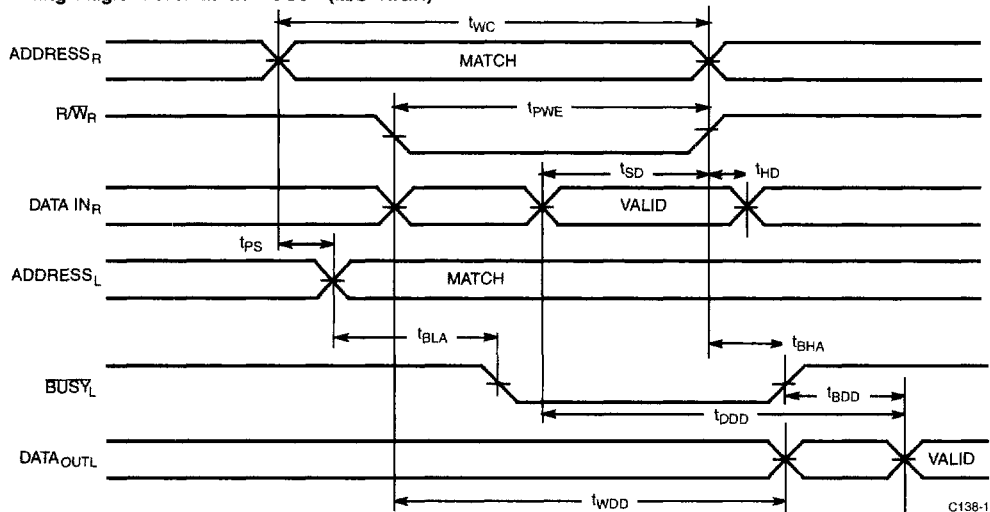
Write Timing with Busy Input ( M/\overline{S}=\text{LOW} )
