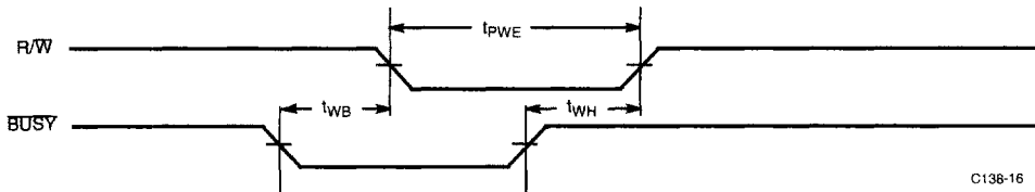
Write Timing with Busy Input ( M/\overline{S}=\text{LOW} )
