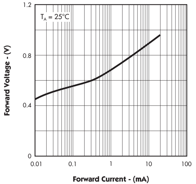
FIGURE 4. — FORWARD CHARACTERISTICS
