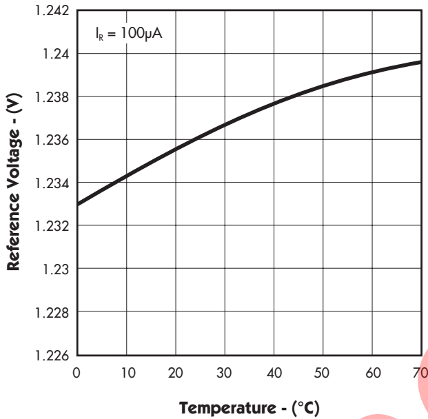
FIGURE 1. — TEMPERATURE DRIFT
