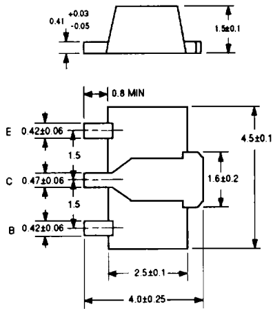
PACKAGE OUTLINE 34 (SOT-89)
