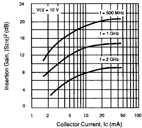
NE85635 INSERTION GAIN vs. COLLECTOR CURRENT
