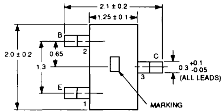
PACKAGE OUTLINE 30 (SOT-323)
