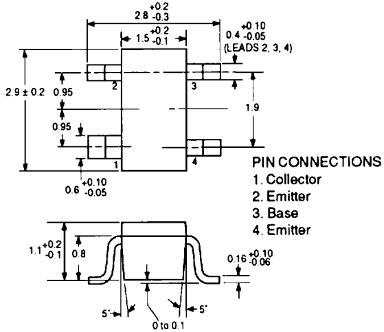
PACKAGE OUTLINE 39
