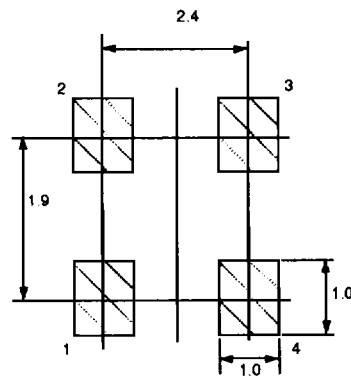
PACKAGE OUTLINE 39 RECOMMENDED P.C.B. LAYOUT
