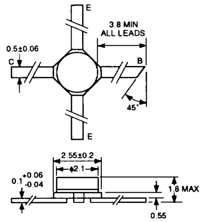
PACKAGE OUTLINE 39 RECOMMENDED P.C.B. LAYOUT
