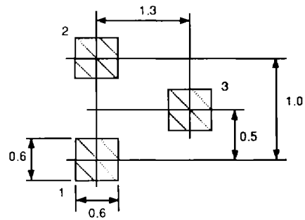
PACKAGE OUTLINE 19 RECOMMENDED P.C.B. LAYOUT
