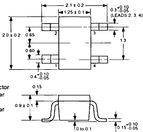
PACKAGE OUTLINE 18 (SOT-343)
