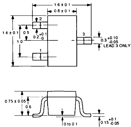
PACKAGE OUTLINE 19
