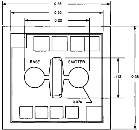
NE85600 (CHIP)
