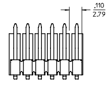
REMOVED BACK WALL OPTION SEE CHART
