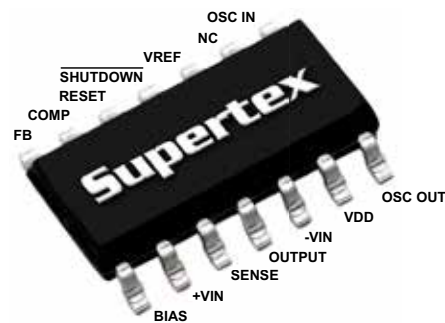
14-Lead SOIC (Narrow Body)
