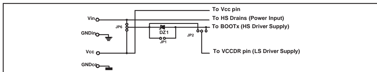
Figure 19. Power supply configuration
