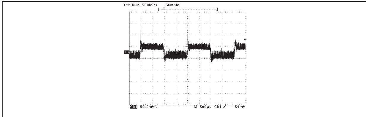
Figure 25. 3A to 45A Load Transient Response
