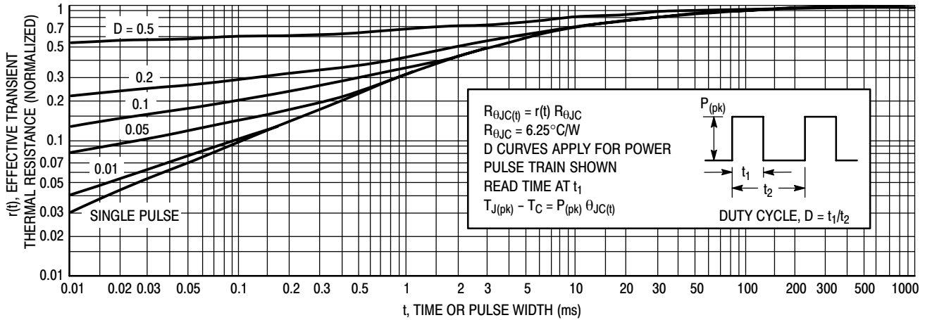
Figure 3. Thermal Response
