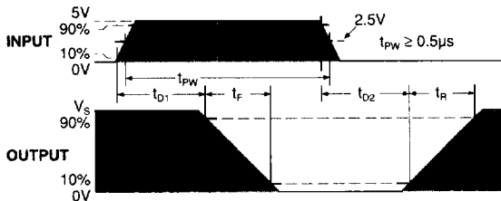
Figure 1a. Inverting Driver Switching Time
