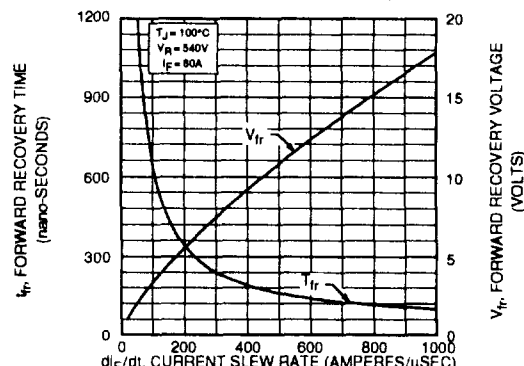
Figure 7, Forward Recovery Voltage/Time vs Current Slew Rate
