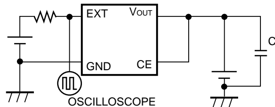
Test Circuit 6
