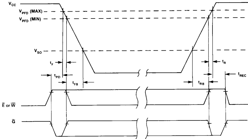
Figure 6. Power-Down/Power-Up Timing
