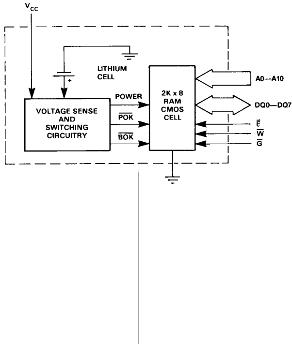
Figure 2. Block Diagram
