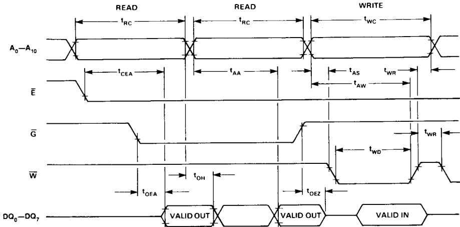
Figure 3. Read-Read-Write Timing
