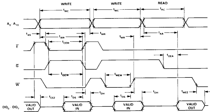
Figure 4. Write-Write-Read Timing
