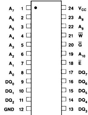
Figure 1. Pin Connections
