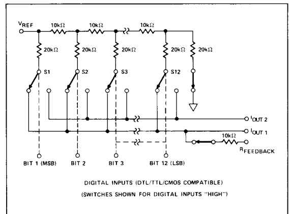
FIGURE 1: Simplified DAC Circuit
