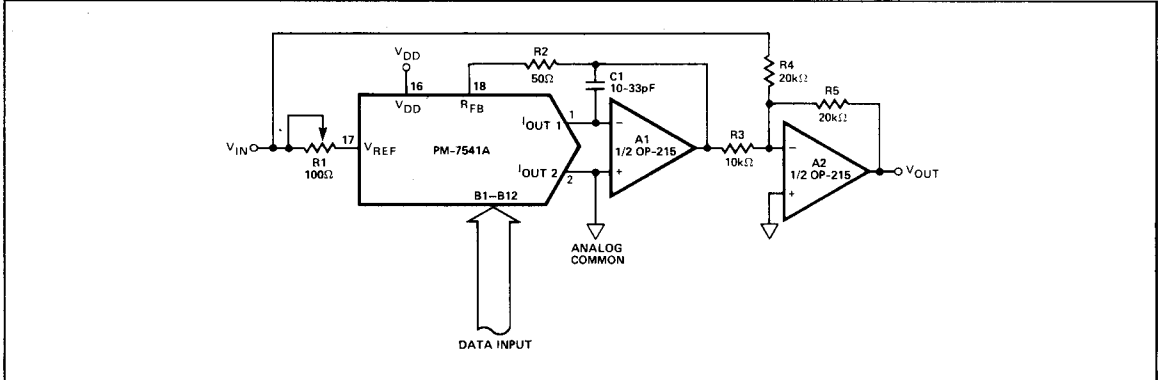
FIGURE 9: Analog/Digital Divider
