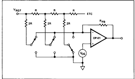
FIGURE 7: Simplified Circuit
