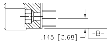
SECTION U-U
