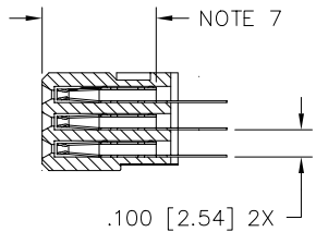
SECTION X-X
