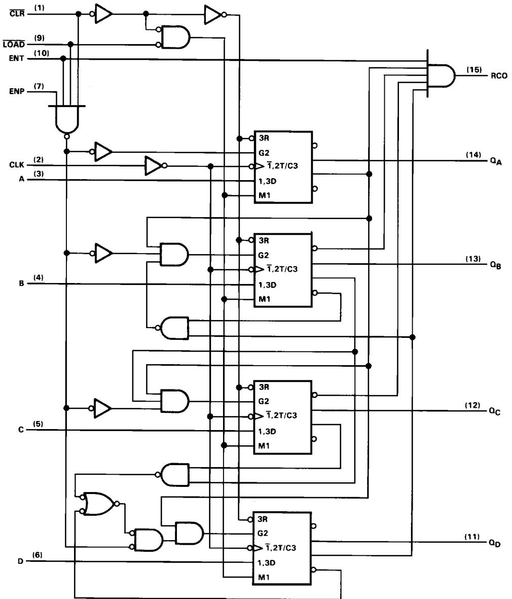
'F162A logic diagram (positive logic)
