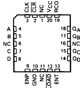
SN54F160A, SN54F162A . . . FK PACKAGE (TOP VIEW)
