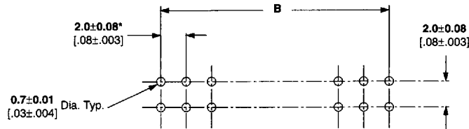
Recommended PC Board Hole Layout * Hole centerline to be 2.0±0.08 [.08±.003]; tolerances not to accumulate within one connector pattern.
