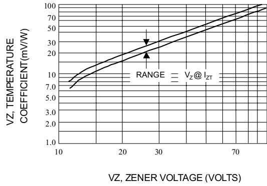
Fig. 2-TEMPERATURE COEFFICIENTS
