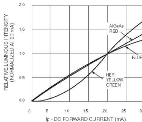
Fig. 2 Relative Luminous Intensity vs. DC Forward Current
