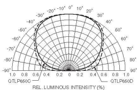
Fig. 4 Radiation Diagram
