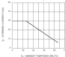
Fig. 5 Maximum Forward Current vs. Ambient Temperature
