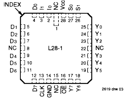
LCC TOP VIEW
